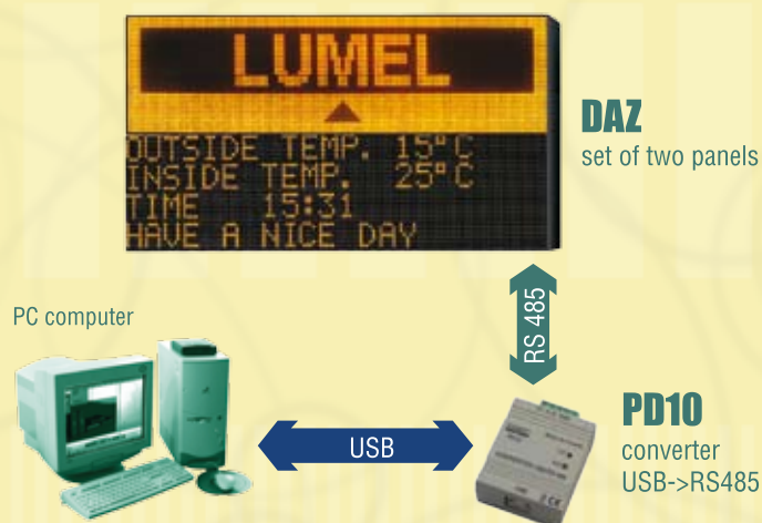
Programming of the DA displays via PD10 USB converter into RS485 Modbus.
