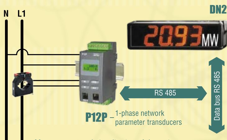
Measurement and visualization of the active power in 1-phase or 3-phase symmetrically loaded network
